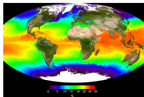
Global Sea Surface Temperature (in IR) from NASA's Terra Satellite. Credit: NASA
